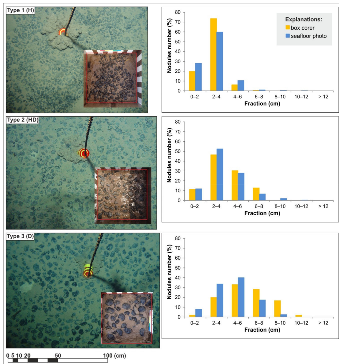
Figure 9. Seafloor and box corer photographs for three genetic types of nodules (left); fraction distributions of nodules defined on the basis of the box corer and seafloor photographs (right).
