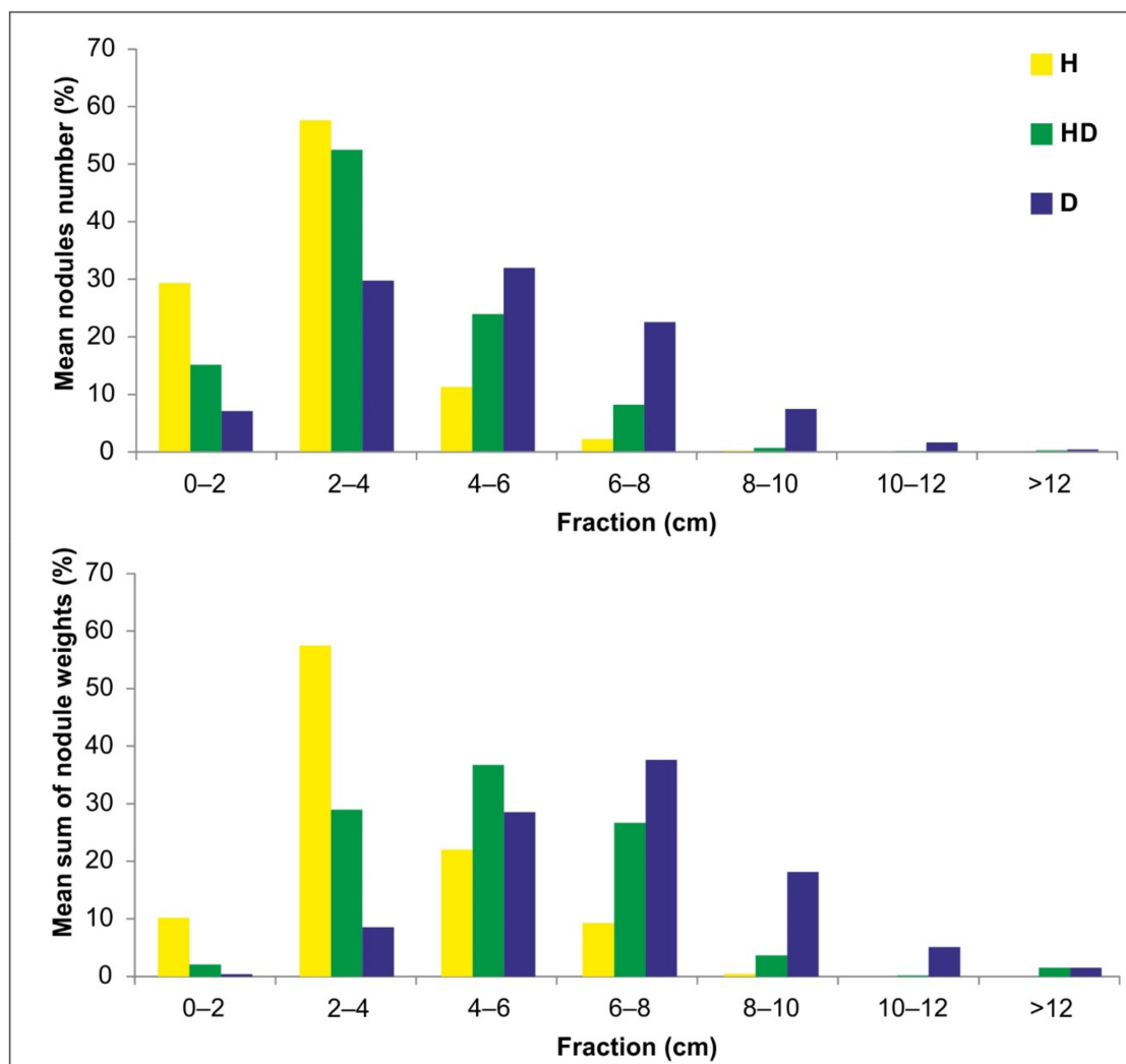
Figure 10. Distributions of the mean number of nodules ( top ) and the mean sum of nodule weights ( bottom ) defined on the basis of the box corer samples from all 68 sampling stations in the H22 exploration block.
